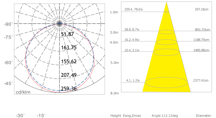
PHOTOMETRIC OF 1M STRIP
