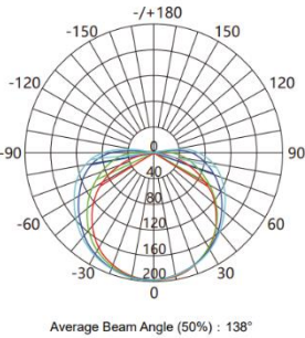
Illuminance Diagram:
